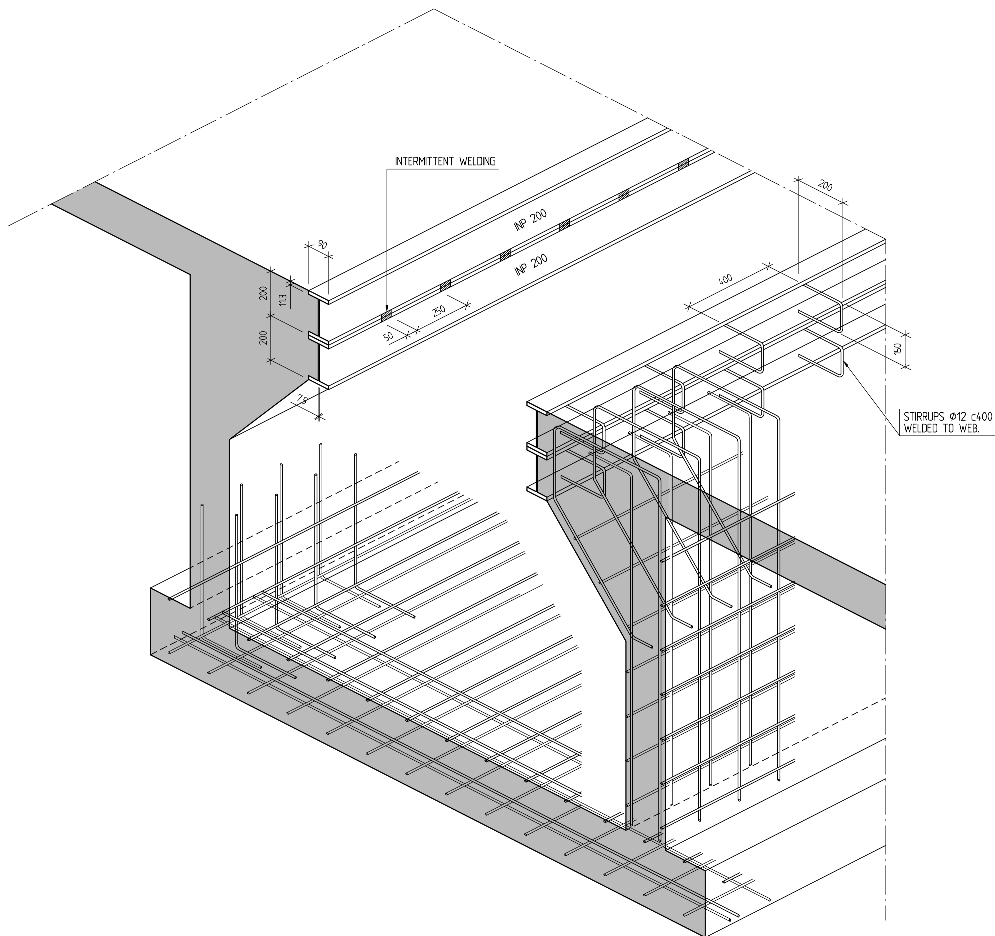
PERSPECTIVE DRAWING 1:10
